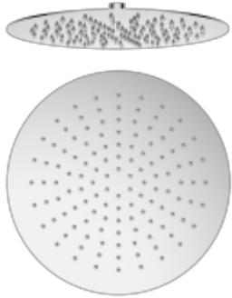
Round Head Shower 12"/Stainless Steel Ø300×2mm
